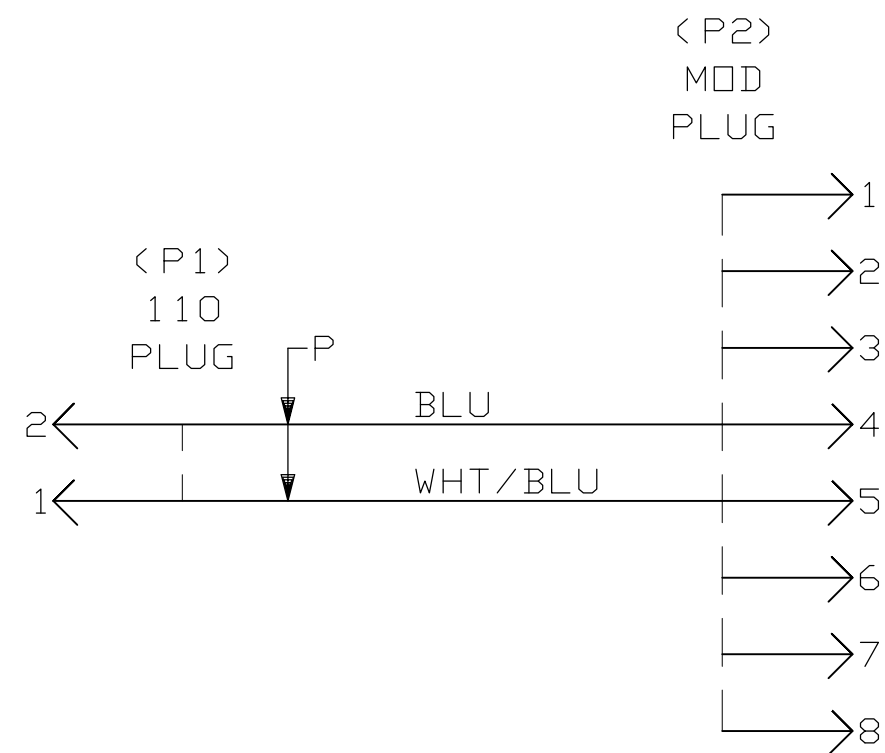
WIRING DIAGRAM
